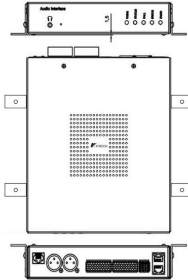
MOUNTING ALTERNATIVE
